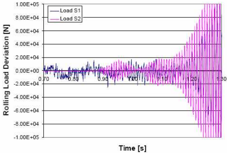
Figure 3: Predictions from a time simulation model showing the rapid onset of third octave chatter involving both stands of a simulated two stand cold tandem mill.
