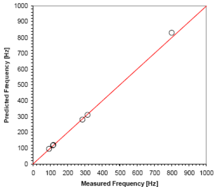
Figure 2: Comparison of predicted and measured mill vibration frequencies for cold mills with different millstand geometries. The straight line represents the condition of predicted frequency being equal to measured frequency.
