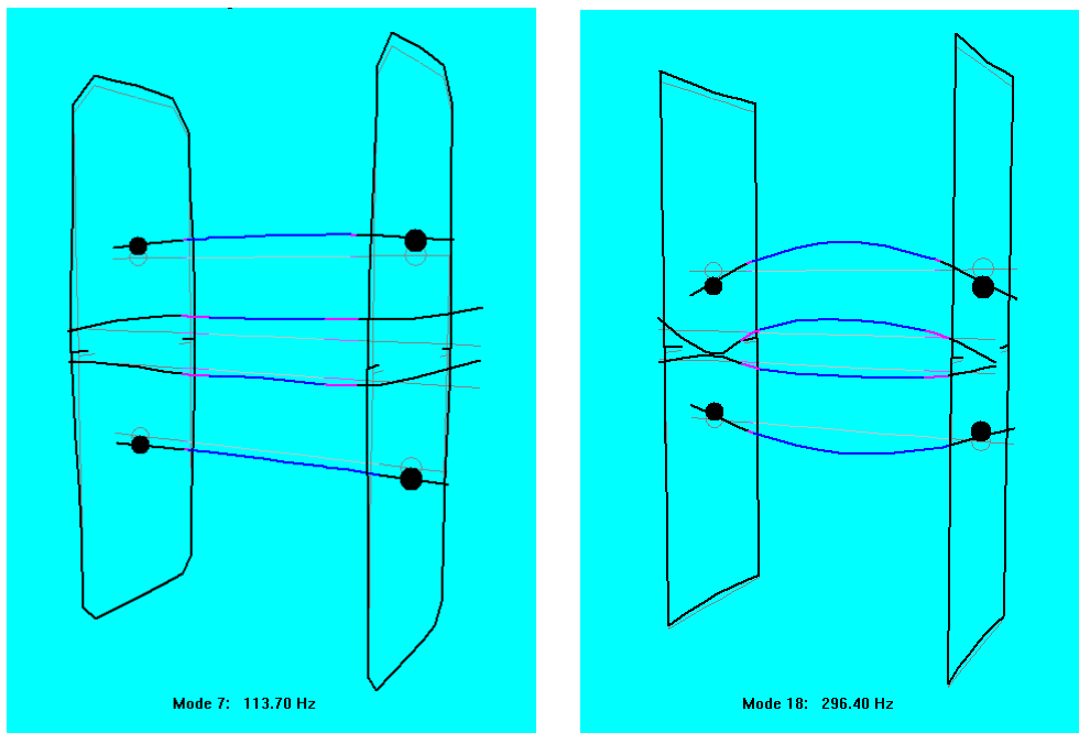
Figure 1: Prediction from the Mill Stand Vibration Model showing a typical gauge chatter vibration mode at 114Hz (left). A less common gauge chatter mode at 296Hz is shown (right) involving significant roll bending.
