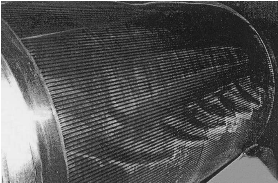
Figure 4: An example of severe fifth octave chatter marks on a back-up roll barrel. The marks are linear and parallel to the roll axis with a regular spacing around the roll circumference.
