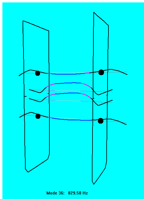
Figure 5: Prediction from the Mill Stand Vibration Model showing a typical fifth octave vibration mode shape for a cold rolling mill
