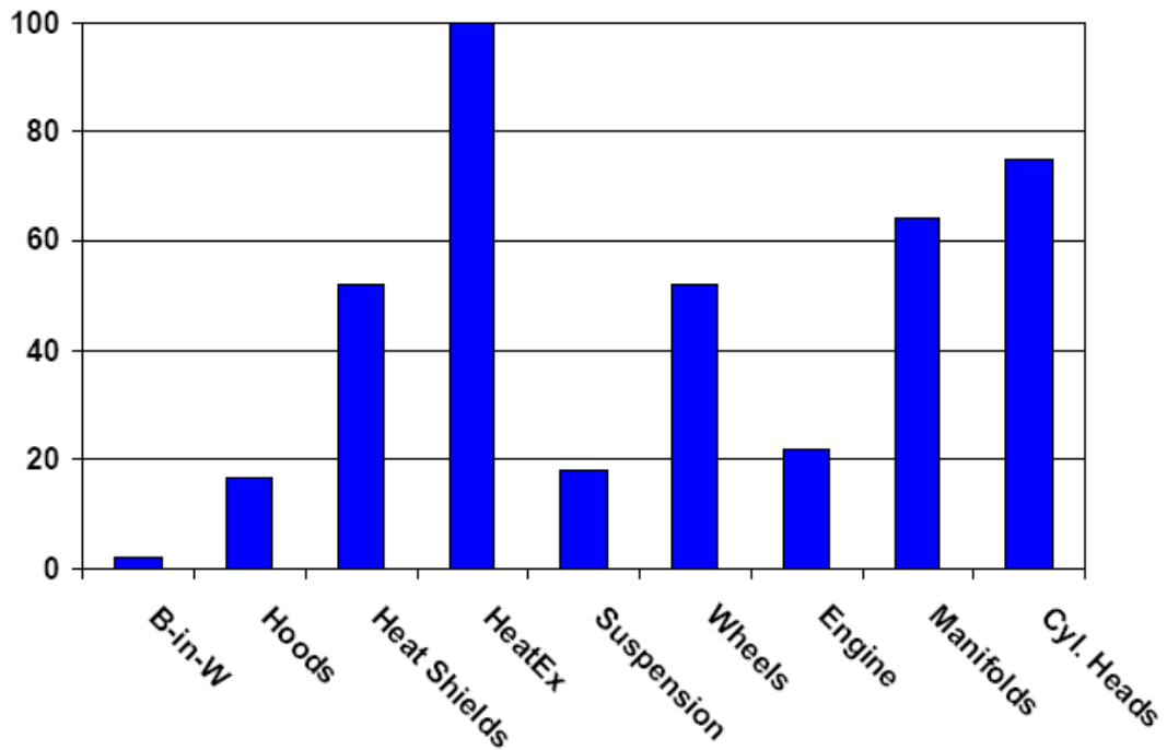
Figure 1 Aluminium Component Penetration % (US): source: Ducker Research
