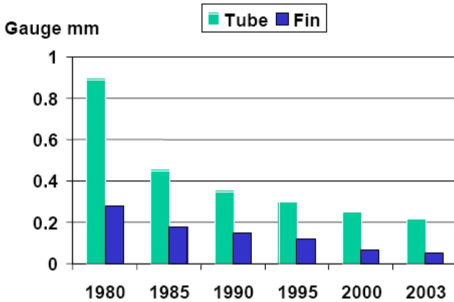
Figure 1 Downgauging trends in tube and finstock alloys
