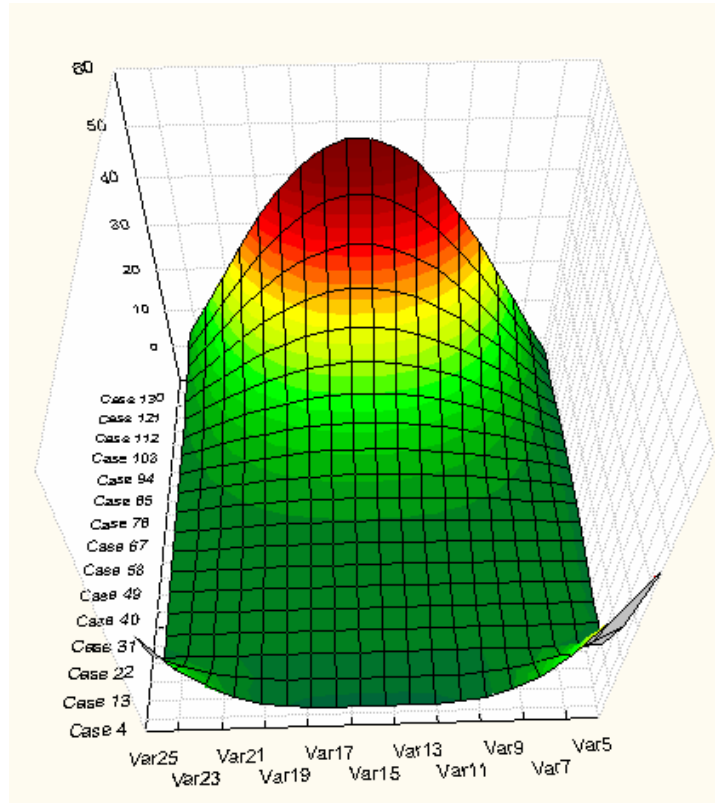
Figure 1: Predicted change in flatness for a coil of a soft aluminium alloy – note the change from spool end to outer lap
