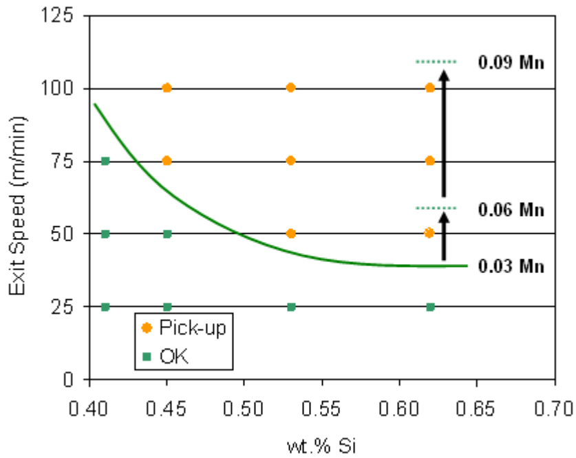
Figure 3: Effect of Si and Mn on onset of surface pick-up.
