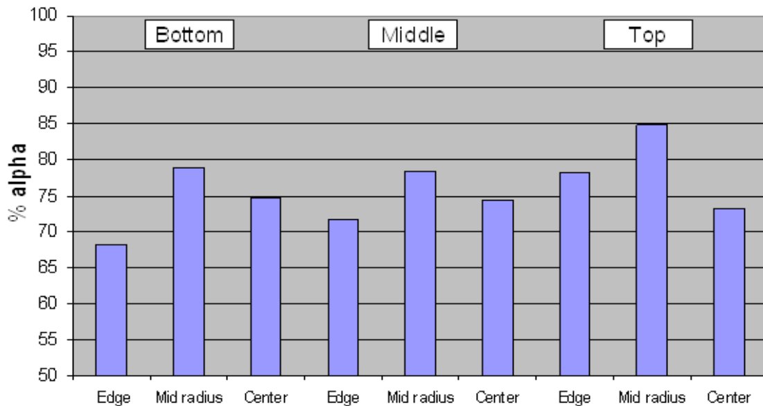
Figure 4: Variation in intermetallics through a homogenised 6063 log.
