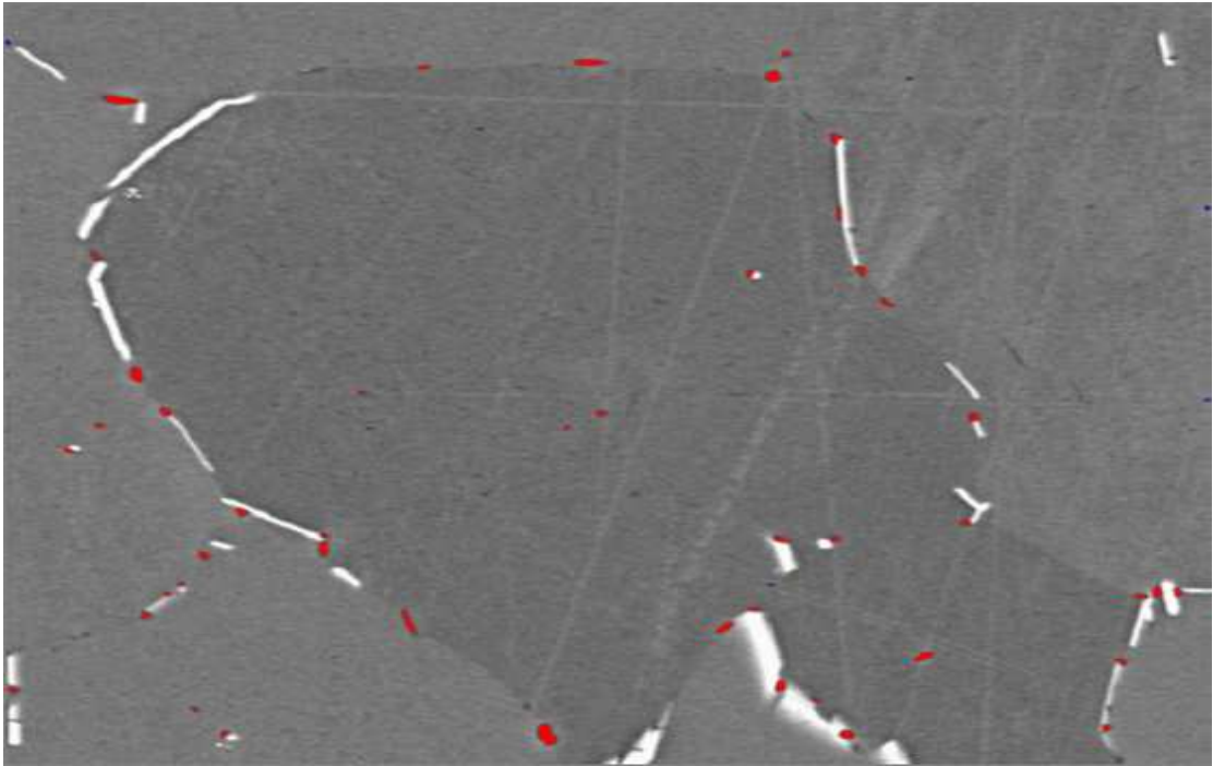
Figure 5: Micrograph showing Mg 2 Si (coloured red) and Fe-rich (white) intermetallics in billet.
