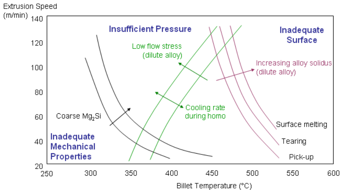
Figure 2: Effect of composition and homogenisation on extrusion window.
