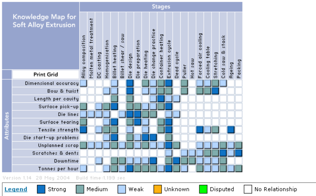
Figure 1: Generic K-Map for a soft alloy extrusion plant using Innoval Technology's proprietary software.
